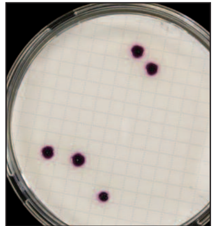
With Modified m-Tec, magenta E. Coli colonies are very easy to see and count.
